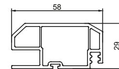
AP 109 SCREEN SASH FOR DOOR
