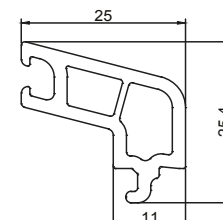
AP 310 GLAZING BEAD FOR SS (6 mm)
