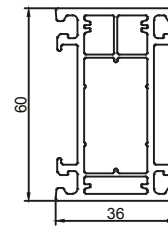
AP 203 UNIVERSAL PROFILE
