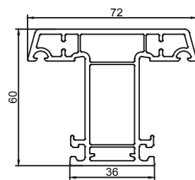
AP 206 T - MULLION
