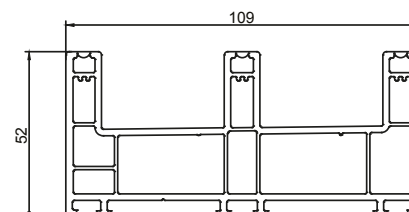
AP 103 SLIDING FRAME 3 TRACK
