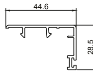
AP 102 SLIDING FRAME WITH MESH TRACK
