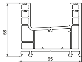
AP 301 SLIDING FRAME 2-TRACK
