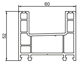
AP 101 SLIDING FRAME 2 TRACK
