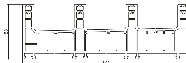
AP 303 SLIDING FRAME 4-TRACK
