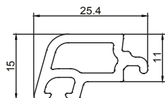
AP 311 DOUBLE GLAZING BEAD FOR SS (18 mm)
