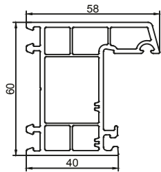
AP 201 CASEMENT WINDOW OUTER FRAME
