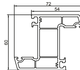
AP 207 Z - MULLION
