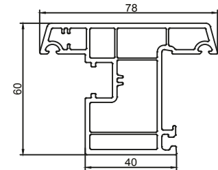
AP 204 CASEMENT WINDOW SASH
