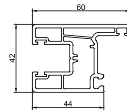
AP 104 SLIDING WINDOW SASH
