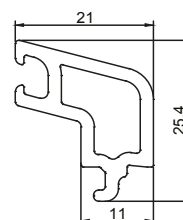
AP 309 GLAZING BEAD FOR SS (10-12 mm)
