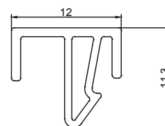
AP 313 MESH LOCK PROFILE
