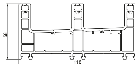
AP 302 SLIDING FRAME 3-TRACK
