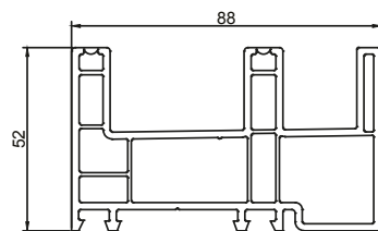
AP 102 SLIDING FRAME WITH MESH TRACK
